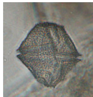
Lingulodinium (dinoflagellate)
