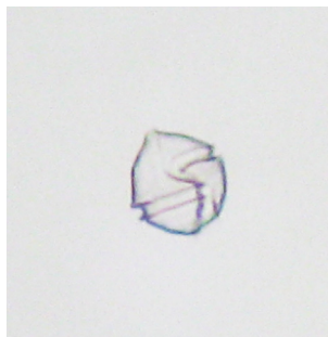
Gonyaulax (dinoflagellate)
